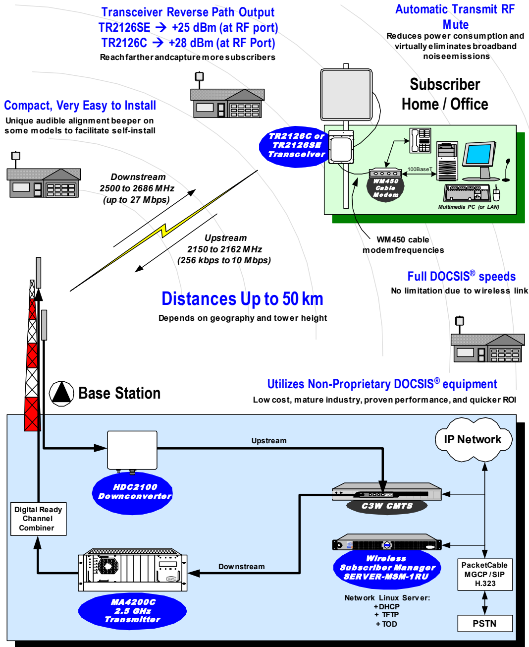
Figure 1: Point-to-Multipoint Overview
